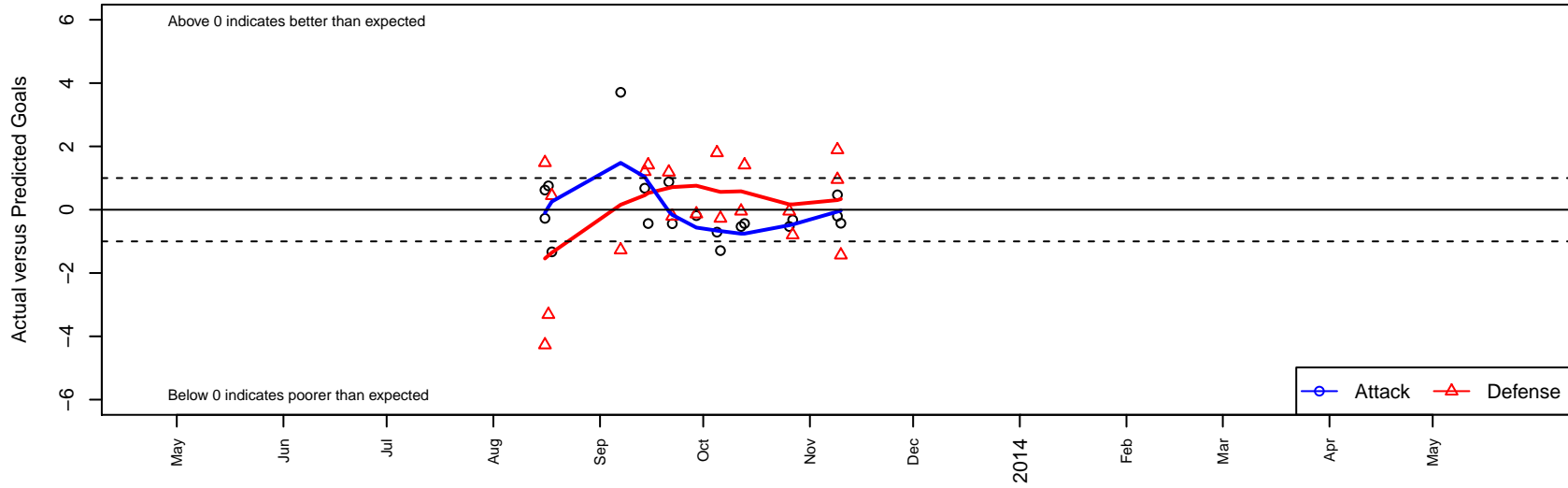
HSC Storm G01 Dots are actual minus expected GF (blue circles) and GA (red triangles). Blue line is smoothed change in attack strength. Red is smoothed change in defense strength.
